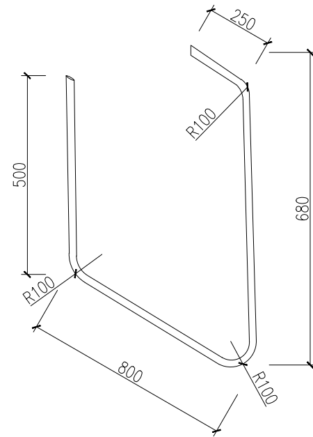
DIMENSION DETAIL OF 6 - 25Ø GAL. PIPE
