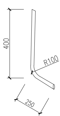
DIMENSION DETAIL OF 9 - 25Ø GAL. PIPE
