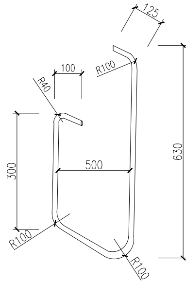
DIMENSION DETAIL OF 8 - 25Ø GAL. PIPE
